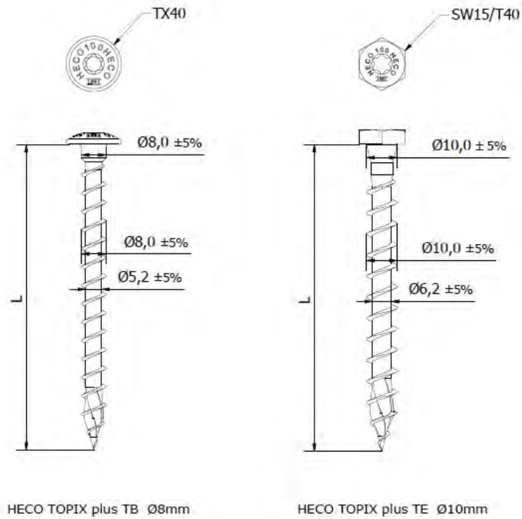
Figure 1: Screws dimension
