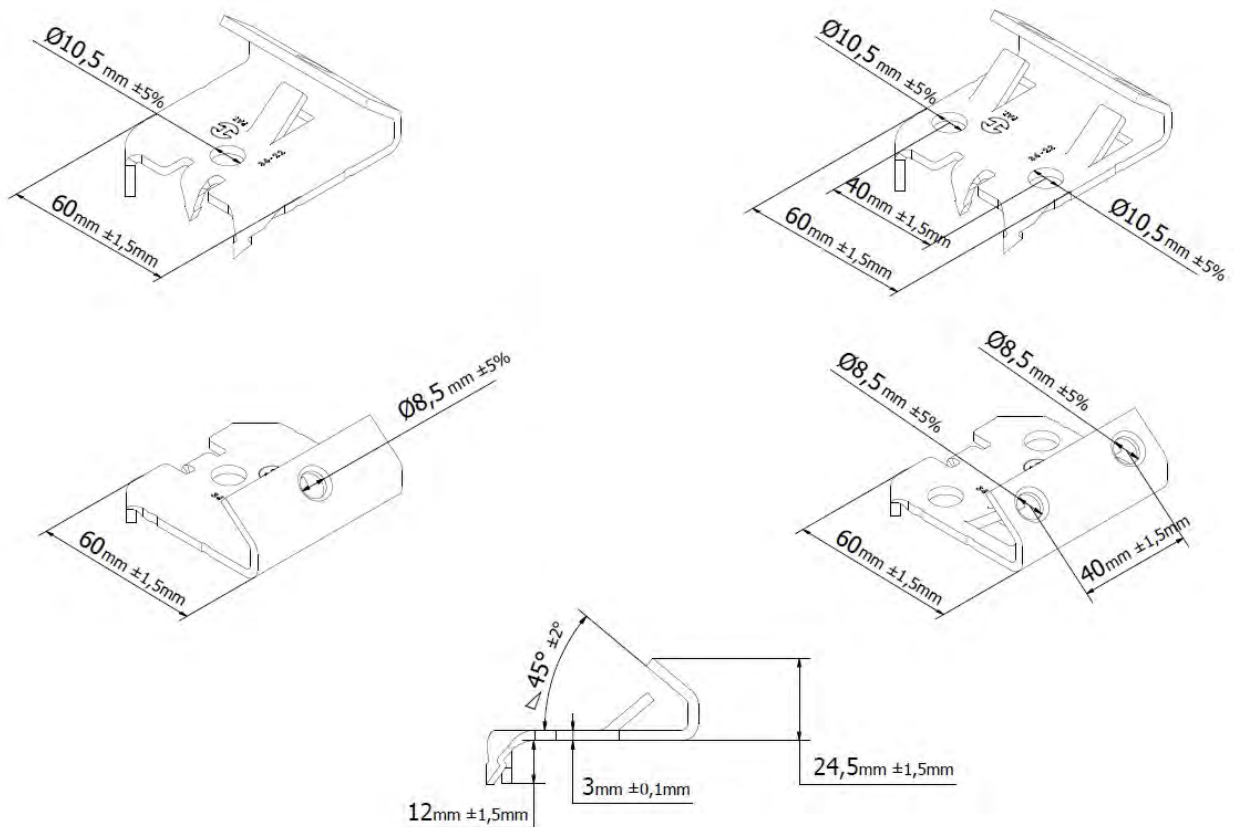
Figure 2: Plate dimension
